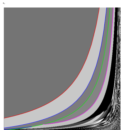
Figure 1: Shows the avalanche type domains on (\epsilon, E_c) -bifurcation diagram for N = 2 . The top domain is E_c > \frac{1+\epsilon}{1-\epsilon} . The line from infinity to the origin is E_c = \frac{\epsilon}{1-\epsilon} . We see infinitely many domains with different avalanches, accumulating to two of the axes.
